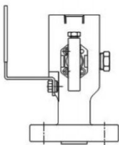
Single block and bleed SB
