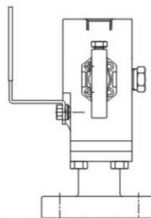
Two Piece Bolted Design P2
